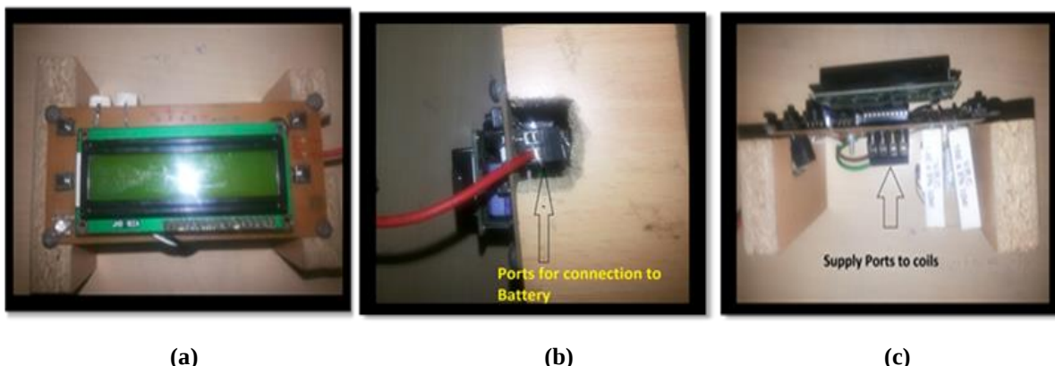
Fig.5 Structure of electromagnetic circuit
