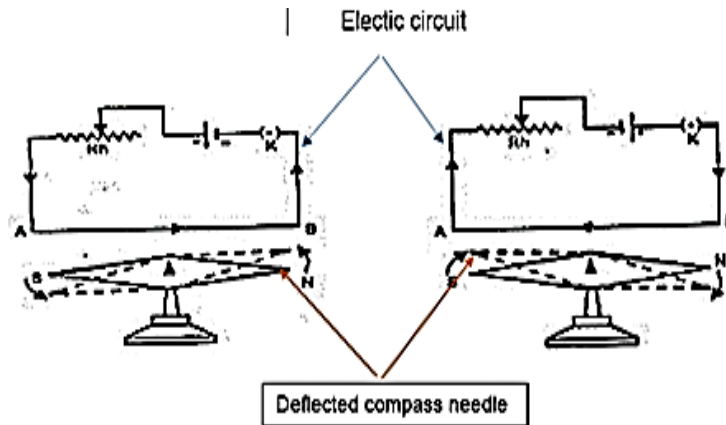
Fig.1.1.1 Oersted law
