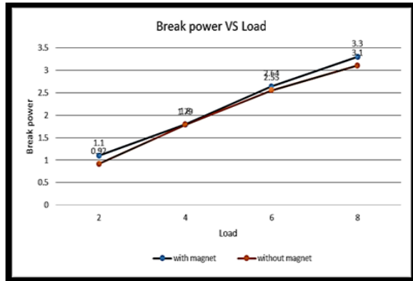
Graph.2 Break power VS load
