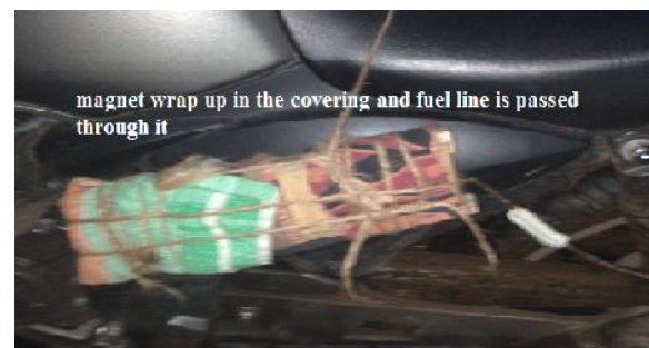
Figure 6. location of permanent magnet and fuel line
